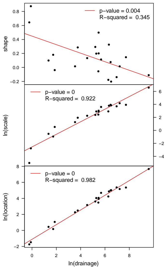
Figure 11: This figure illustrates the relationships between the site-specific maximum likelihood GEV parameter estimates and their corresponding drainage area. Also shown are the regression lines for the corresponding three linear regression models. For each plot, the two sided t-test on the regression slope and the associated R-squared are also given.
